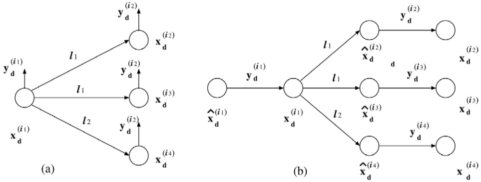
Fig. 2. Moore-automaton (left) and an equivalent automaton without outputs (right). Note that y_d^{(ik)} = \mu(x_d^{(ij)}) \in Y_d is the output symbol associated with the discrete state x_d^{(i)} .
