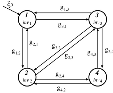
Fig. 1. A graph describing a hybrid automaton.
