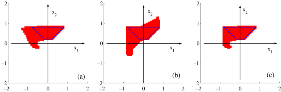
Fig. 6. Invariants (in white) of locations 1 (a) and 2 (b) and (c) the forbidden region X_f = X \setminus (\text{inv}_1 \cup \text{inv}_2) defined in Definition 4.9. The interior of the blue trapezoid is the forbidden region X_d .
