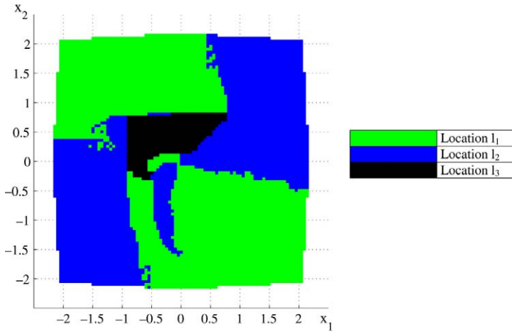
Fig. 7. Switching table of the problem \overline{OP}(\overline{HA}) defined in the example.
