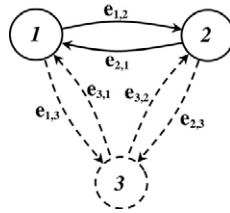
Fig. 4. Graph of the automaton HA (continuous) and \overline{HA} (continuous and dashed) described in the example.
